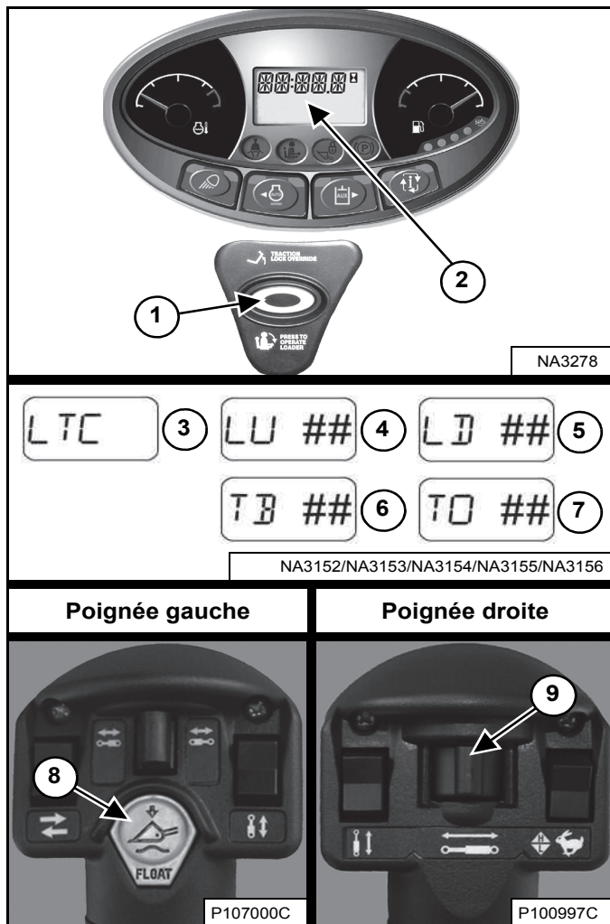
Figure 77
