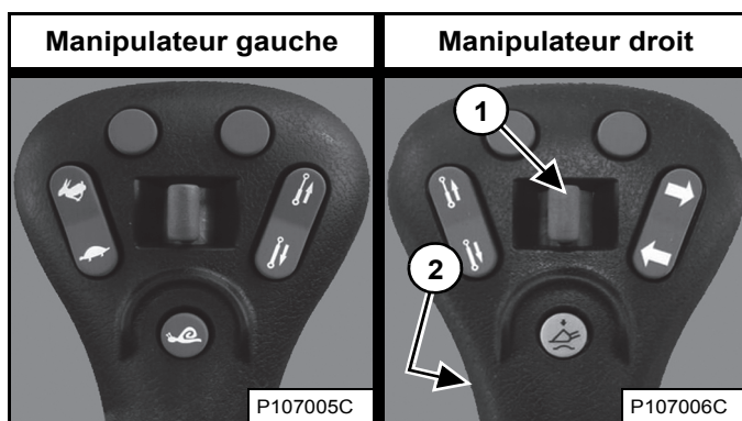
Figure 95
