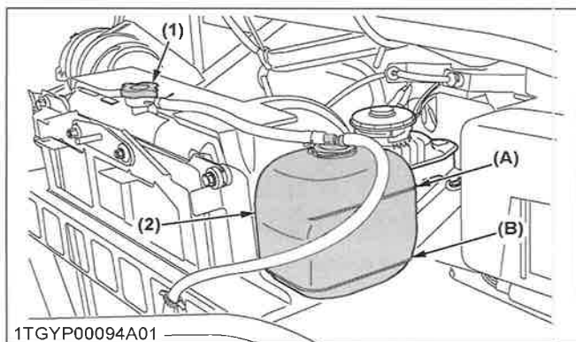
(1) Radiateurdop
